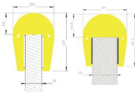
8mm PROTECTOR
