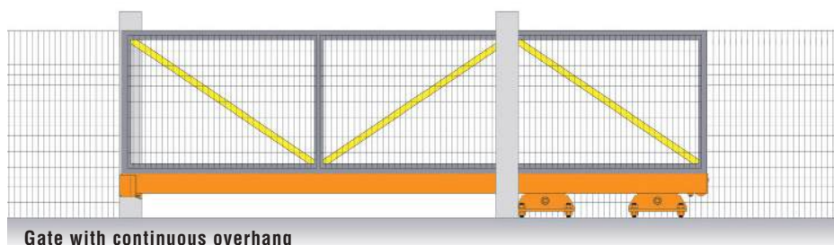
Gate with continuous overhang
