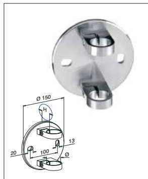
FIXED SLAB BRACKET
