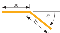
Ramp Bend
